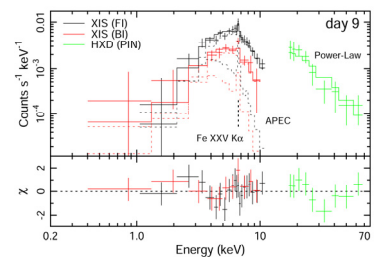
Fig.3. Background-subtracted spectra (cross) and the best-fit model on day 9. The best-fit models are shown by the solid (total) and dashed (each component) histograms.
