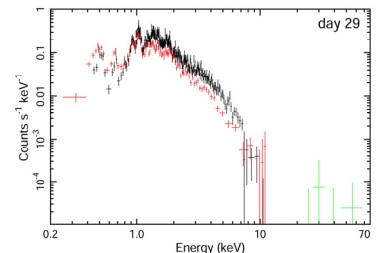
Fig.4. Background-subtracted spectra (cross) on day 29.
